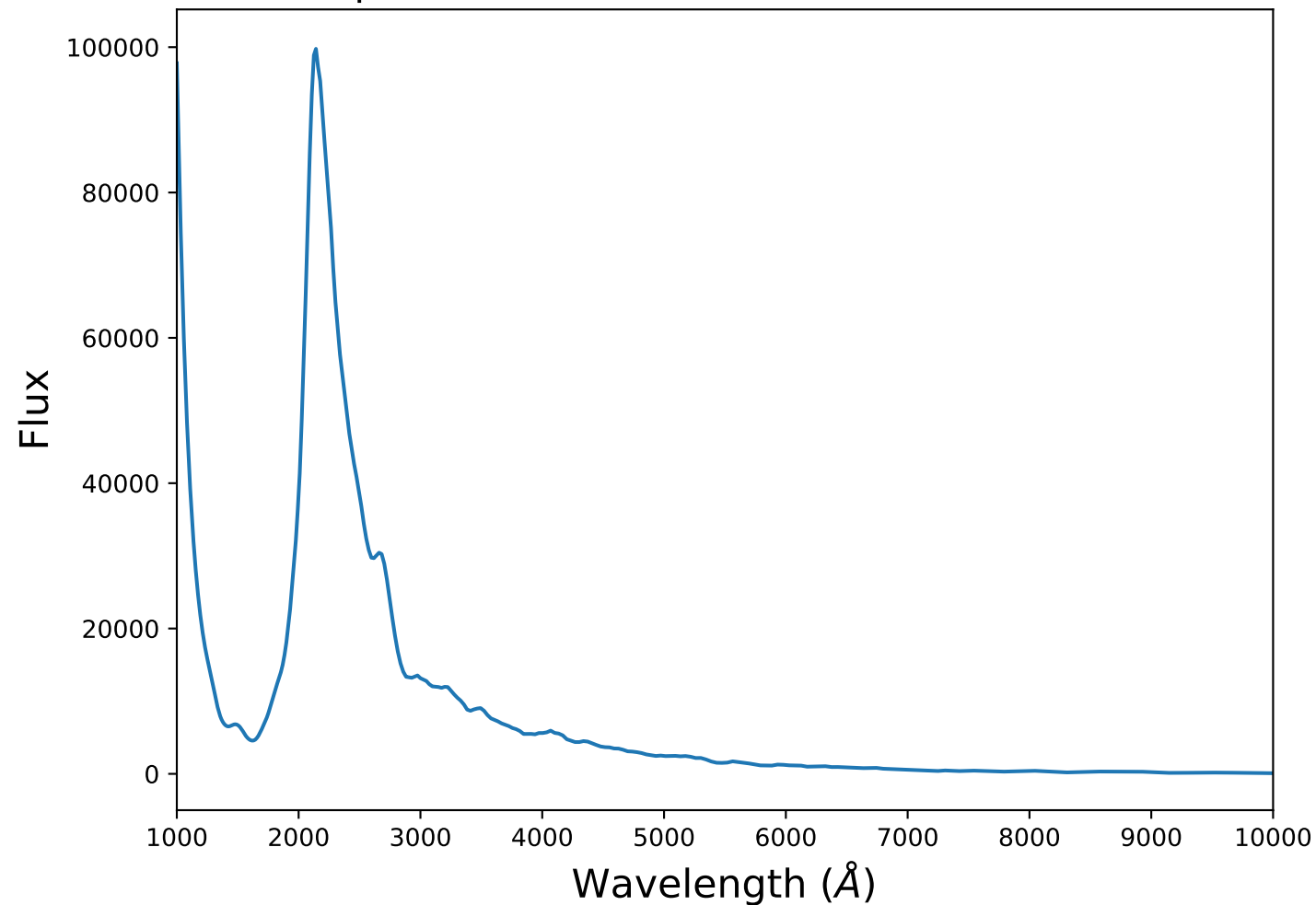
Spectrum 1 for transient SNIa at z=0.40
